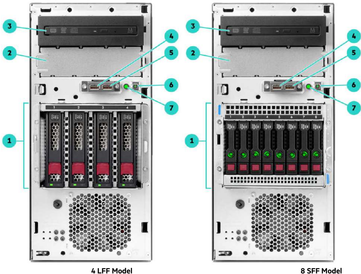
Front View (details for 4LFF and 8SFF)
