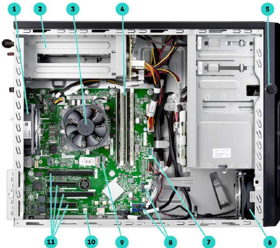
Internal View
